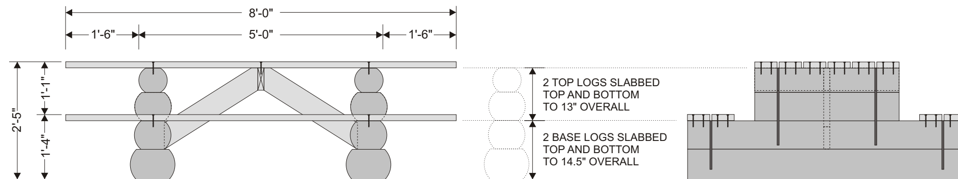
SIDE VIEW
